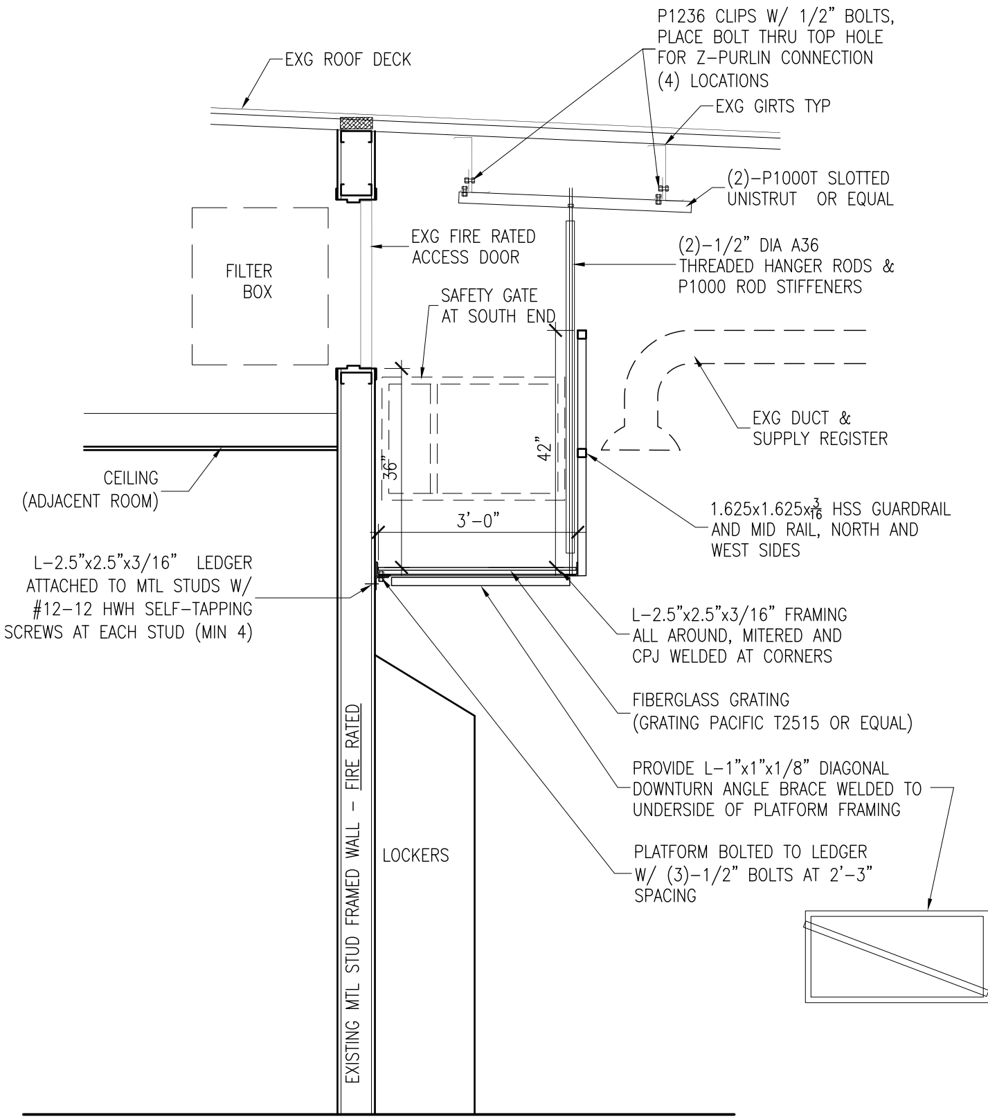
SECTION OF FILTER ACCESS PLATFORM 1/2" = 1'-0"
