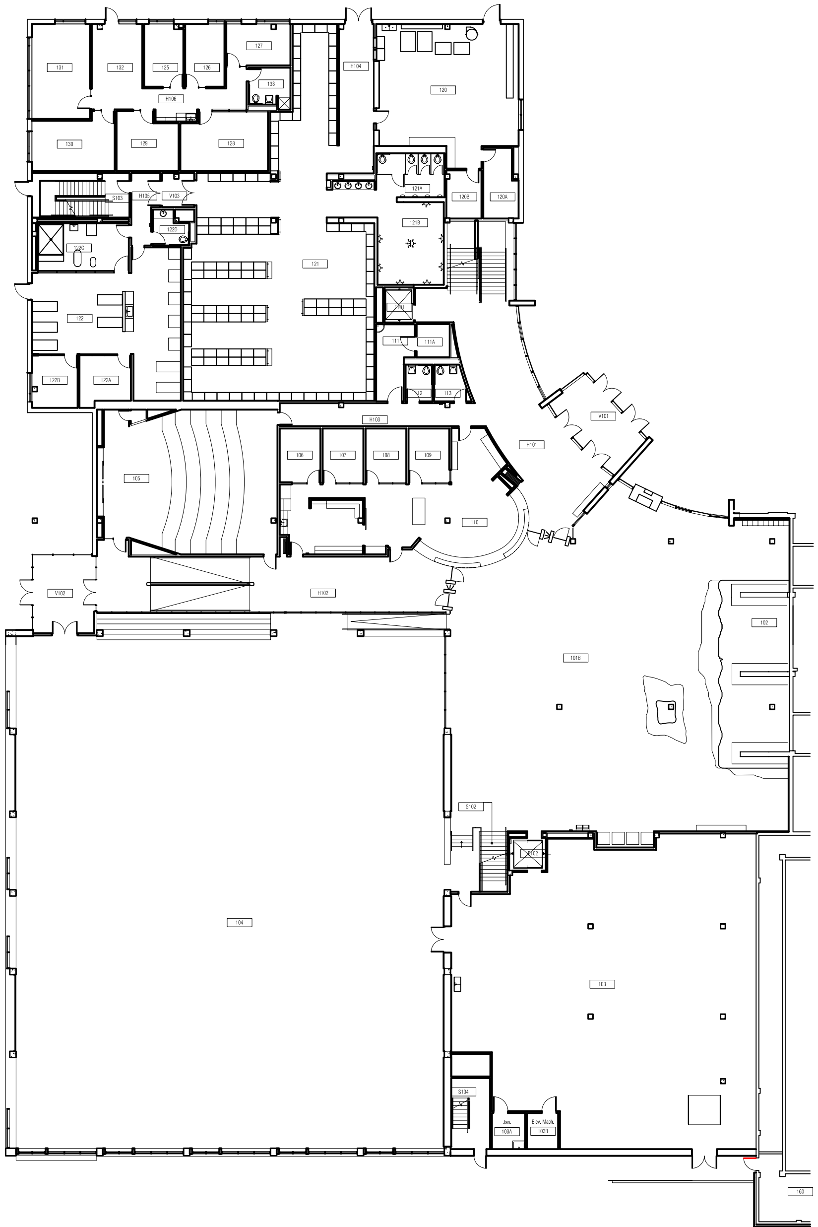
WESTERN OREGON UNIVERSITY HEALTH & WELLNESS CENTER 1 LEVEL AND FOOTBALL AREAS
